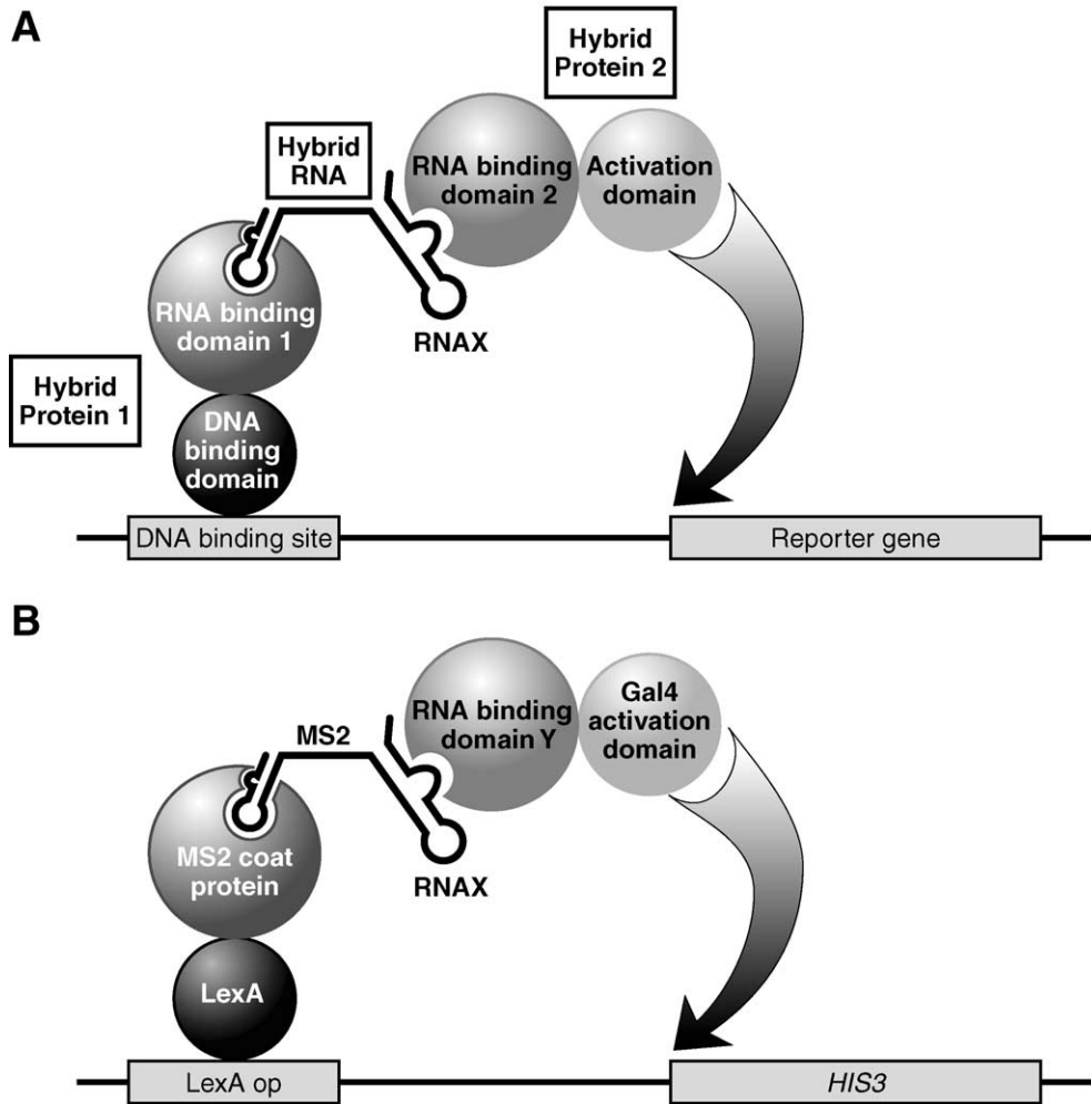
Fig. 1. Three-hybrid system to detect and analyze RNA–protein interactions. (A) General strategy of the system, (B) Specific protein and RNA components that typically have been used to date. Other RNA and protein components also can be used (see text). For simplicity, the following features are not indicated. Both lacZ and HIS3 are present in strain L40coat and YBZ-1 under the control of lexA operators, and so can be used as reporters. Multiple LexA operators are present (four in the HIS3 promoters and eight in the lacZ promoter), and LexA protein binds as a dimer. The hybrid RNA contains two MS2 binding sites, and MS2 coat protein binds as a dimer to a single site. Adapted, with permission from SenGupta et al. [1].
