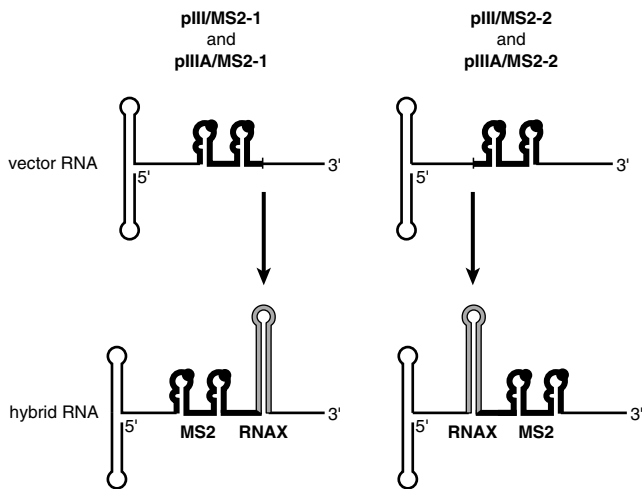
Fig. 3. Schematic diagram of the secondary structure of the hybrid RNA molecules. Thin lines: RNase P RNA 5' leader and 3' trailer sequences; bold lines: tandem MS2 recognition sites, including a point mutation that increases affinity (black dot); gray lines: inserted RNA sequence, depicted as a stem-loop.
