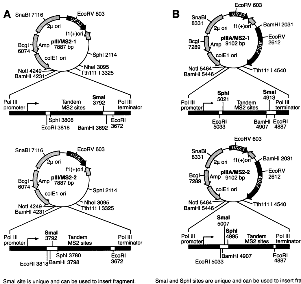
Fig. 2. Plasmid vectors used to express hybrid RNAs in the three-hybrid system. The restriction sites that are indicated either are unique or can be used to verify the presence of various elements on the plasmids. Sites suitable for insertion of sequences of interest are in boldface.
