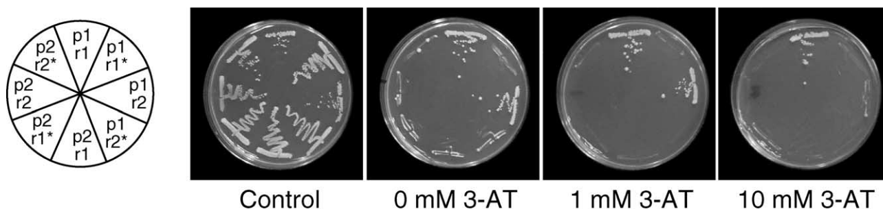
Fig. 6. RNA–protein interactions monitored by level of resistance to 3-AT. A sample growth assay on medium lacking histidine and containing 3-AT. The first plate is a control plate (–ura, –leu) demonstrating that all combinations are viable in the absence of selection for HIS3 . The second, third, and fourth plates lack histidine and contain 0, 1, and 10 mM 3-AT, as indicated. Protein p1 interacts strongly with RNA r1 and moderately with RNA r2, but not with mutated RNAs, r1* and r2*. A related protein, p2, does not interact with either RNA.
