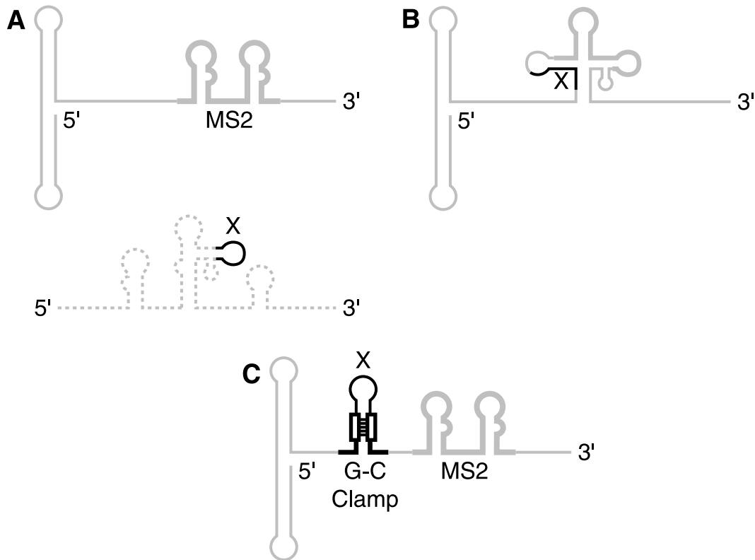
Fig. 4. “GC clamps” in a hybrid RNA molecule. A schematic diagram of the secondary structure of hybrid RNA molecules with and without the GC clamp. The RNA sequence that is being analyzed is a short stem-loop, X, indicated by a thin black line. Thin gray lines: RNase P RNA 5' leader and 3' trailer sequences; thick gray lines: tandem MS2 recognition sites; dashed gray lines: the natural RNA sequence in which RNA X resides; thick black line with boxes: “GC clamp.” (A) Top: predicted structure of hybrid RNA vector sequence; bottom: RNA X in its natural context. (B) When inserted into the hybrid RNA (depicted in A), the new chimeric RNA (depicted in B) adopts a structure in which neither the stem-loop X nor the MS2 binding sites fold properly. (C) To restore the proper conformation, a GC clamp is inserted. See Ref. [25] for details.
