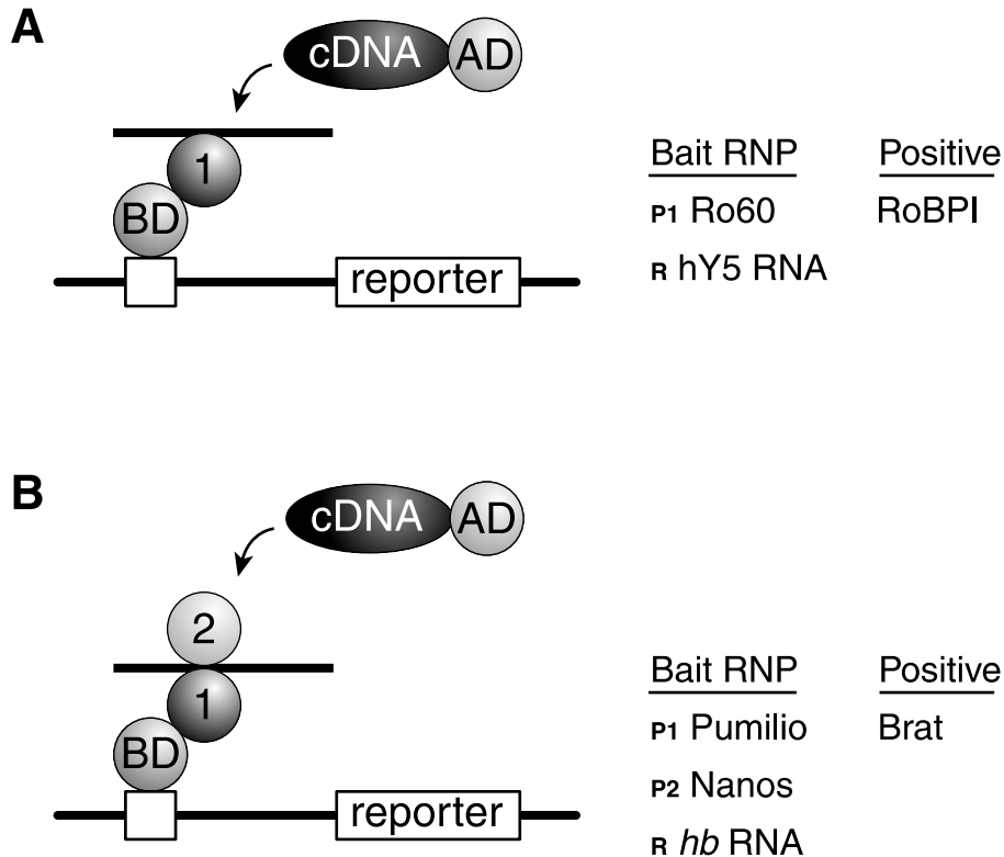
Fig. 8. Screens to identify proteins in multicomponent complexes: RNP “baits.” Strategies used to look for multicomponent RNPs using the three-hybrid system. (A) A screen for proteins that interact with a protein–RNA complex. The DNA binding domain is fused to an RNA binding protein of choice (1) to tether the RNA. This was used by Bouffard et al. [17] to find proteins that interact with Ro60 protein bound to hY5 RNA. (B) A screen for a proteins that interact with a ternary protein–RNA complex. The DNA binding domain is fused to an RNA binding protein of choice (1) and a nonhybrid protein (2) is supplied to form the ternary complex with the RNA. This configuration was used by Sonoda and Wharton [42] to find proteins that interact with a ternary complex of Pumilio, Nanos, and hunchback RNA.
