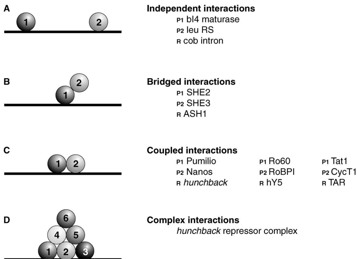
Fig. 7. Analyzing multicomponent complexes. A diagram of four permutations of complexes involving one RNA and two or more proteins. Each type of permutation has been analyzed in the three-hybrid system. Relevant citations are: (A) Ref. [19]; (B) Ref. [30]; (C) Refs. [16,17,40,41]; and (D) Ref. [42]. See text for details.
