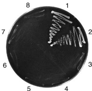
Fig. 5. IRE/IRP1 interaction monitored by activation of the HIS3 . Plasmids encoding the indicated hybrid RNAs and activation domain fusions were transformed into strain L40coat. After selecting transformants for the presence of the plasmids, colonies were assayed for HIS3 reporter activity. Only the two combinations that should lead to IRE–IRP1 interactions (lines 1 and 2) yield growth on media lacking histidine.
